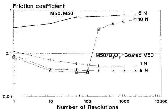
Fig. 1. Friction coefficients of M50–M50 pairs with and without boric oxide coatings under loads of 1, 5, and 10 N as a function of the number of revolutions.
