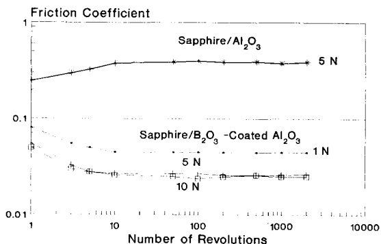
Fig. 2. Friction coefficients of sapphire–alumina test pairs with and without boric oxide coatings under loads of 1, 5, and 10 N as a function of the number of revolutions.
