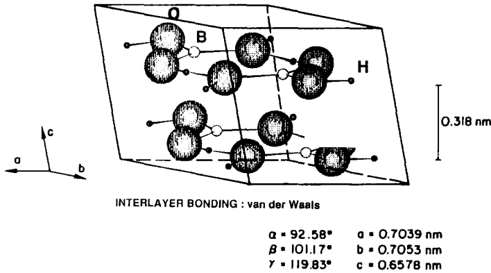
Fig. 5. Depiction of unit cell and cell parameters of bulk boric acid.
